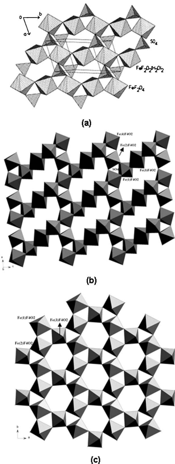
Fig. 3 (a). Fusion of butlerite-type chains to form the layered structure in [\text{M}_2\text{F}_2(\text{SO}_4)_2(\text{H}_2\text{O})_2]_n^{2n-} , X , ( \text{M} = \text{Fe}, \text{Mn} ) from ref. 17. (b) Layered in [\text{Fe}_2^{\text{III}}\text{Fe}_3^{\text{II}}\text{F}_{12}(\text{SO}_4)_2(\text{H}_2\text{O})_2]^{4-} , XI , with symmetrical capping of the sulfate tetrahedra in the triangular lattice and the 10-membered aperture within it, redrawn from ref. 60. (c) Polyhedral view of the kagome layer in XII , from ref. 60.
